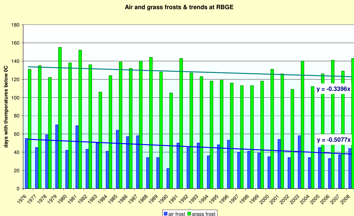
Figure 1. Days of air and grass frosts at RBGE Inverleith site.
